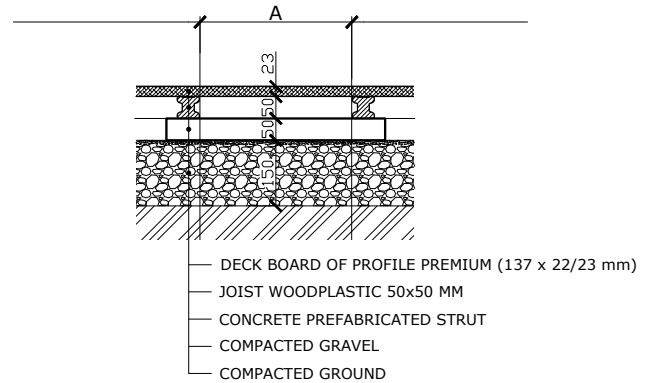
Pic. 1 - Composition of WoodPlastic® decking, including joists 50 x 50mm.
