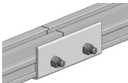
COUPLING - JOIST 40
